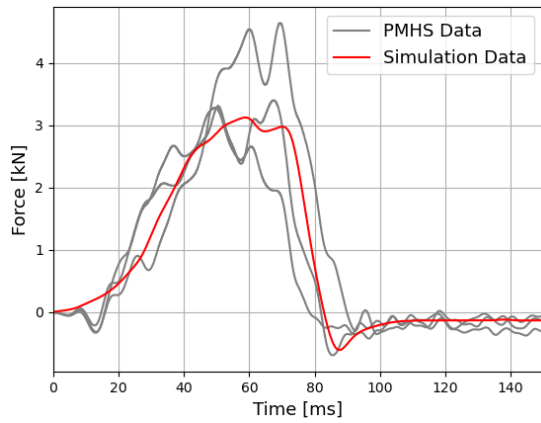
C: Seatpan forces in X-direction
