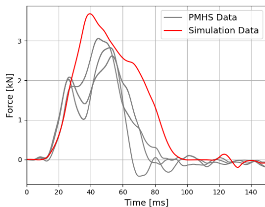
G: Footrest forces in X-direction
