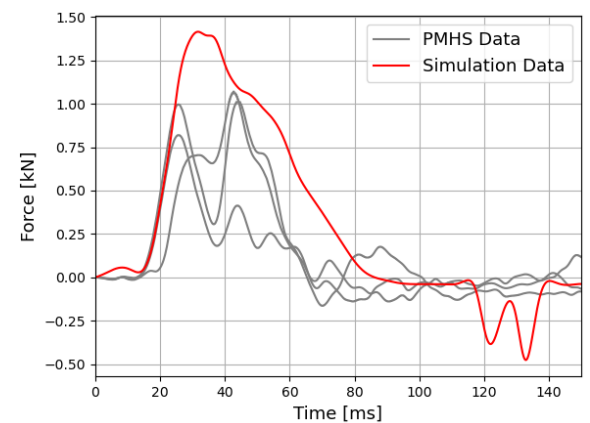
H: Footrest forces in Z-direction
