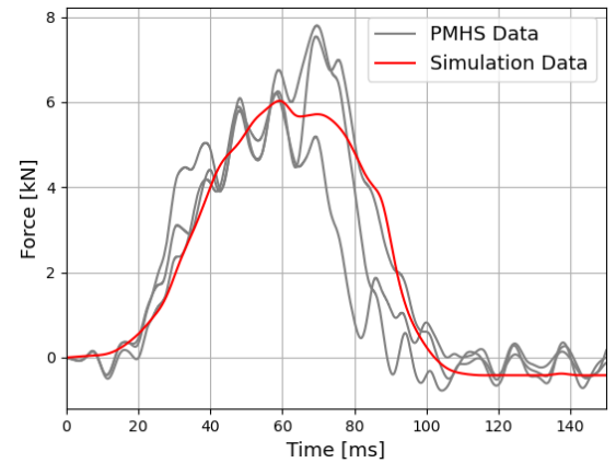
D: Seatpan forces in Z-direction
