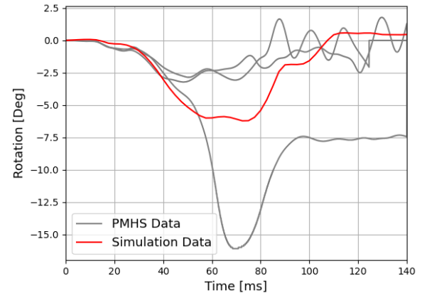
F: Anti submarining guards rotation around the Y-axis
