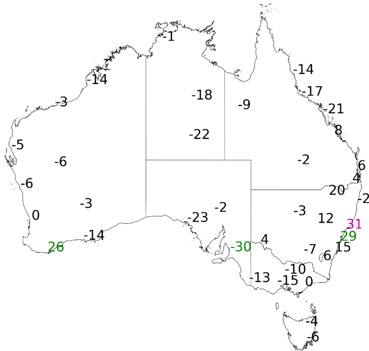
S1 Fig. Partial correlation coefficient values multiplied by 100 for DJF 90 th percentile FFDI and a. JJA NINO3.4 b. JJA SAM c. JJA IOD (two season lag) (1972 – 2017). Significance greater than 99% in red, 95% in magenta and 90% green.
