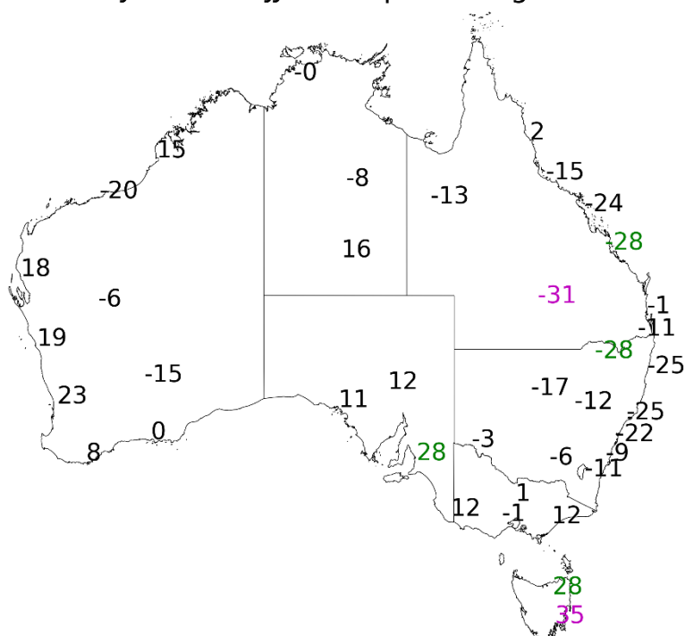
S1 Fig. Correlation coefficient values multiplied by 100 calculated for SON 90 th percentile FFDI and the preceding a. JJA SAM (one-season lag) b. MAM SAM (two-season lag) c. DJF 90 th percentile FFDI and the preceding JJA SAM (two-season lag). Significance greater than 99% in red, 95% in magenta and 90% green.
