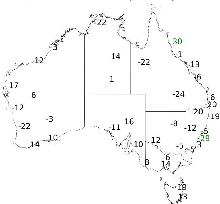
S2 Fig. Correlation coefficient values multiplied by 100 calculated for JJA 90 th percentile FFDI and the preceding MAM NINO3.4 (one-season lag). Significance greater than 99% in red, 95% in magenta and 90% green.
