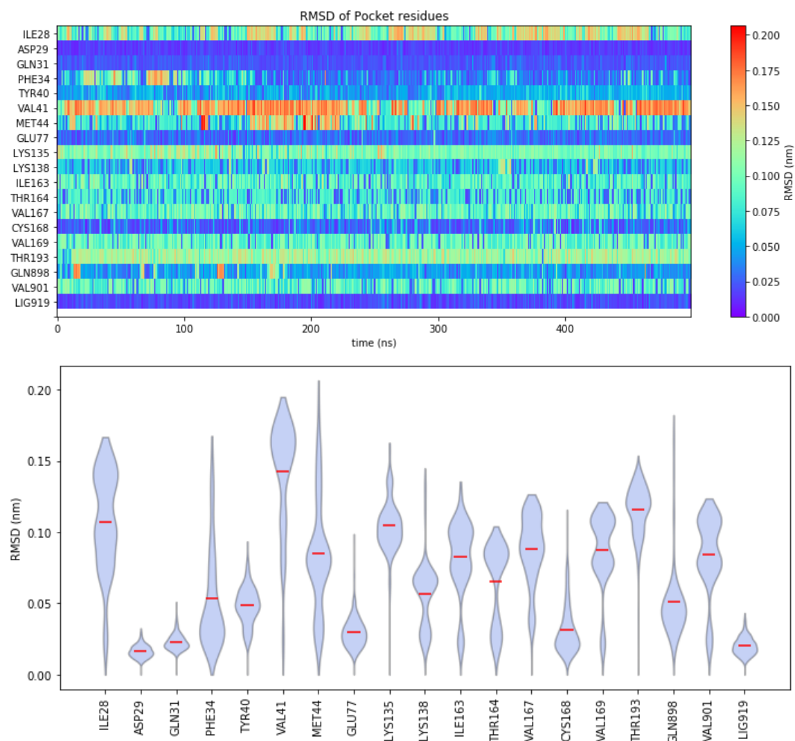
S8 Fig. Root mean square distance for BiuH active site and biuret during molecular dynamics simulation. Top: Root mean square distance from the crystallographic conformation for active site residues and biuret over the course of a 500 ns molecular dynamics simulation. Bottom: Distributions of root mean square distances from the crystallographic conformation for active side residues during a 500 ns molecular dynamics simulation.
