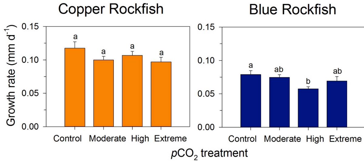
S3 Fig. Growth rates ( \text{mm d}^{-1} ) measured as a change in length over the experimental exposure duration for copper and blue rockfish as a function of p\text{CO}_2 treatment history. Bars are mean values ( \pm SE). Letters over bars represent results of Tukey HSD post-hoc tests; significantly different means do not share letters in common.
