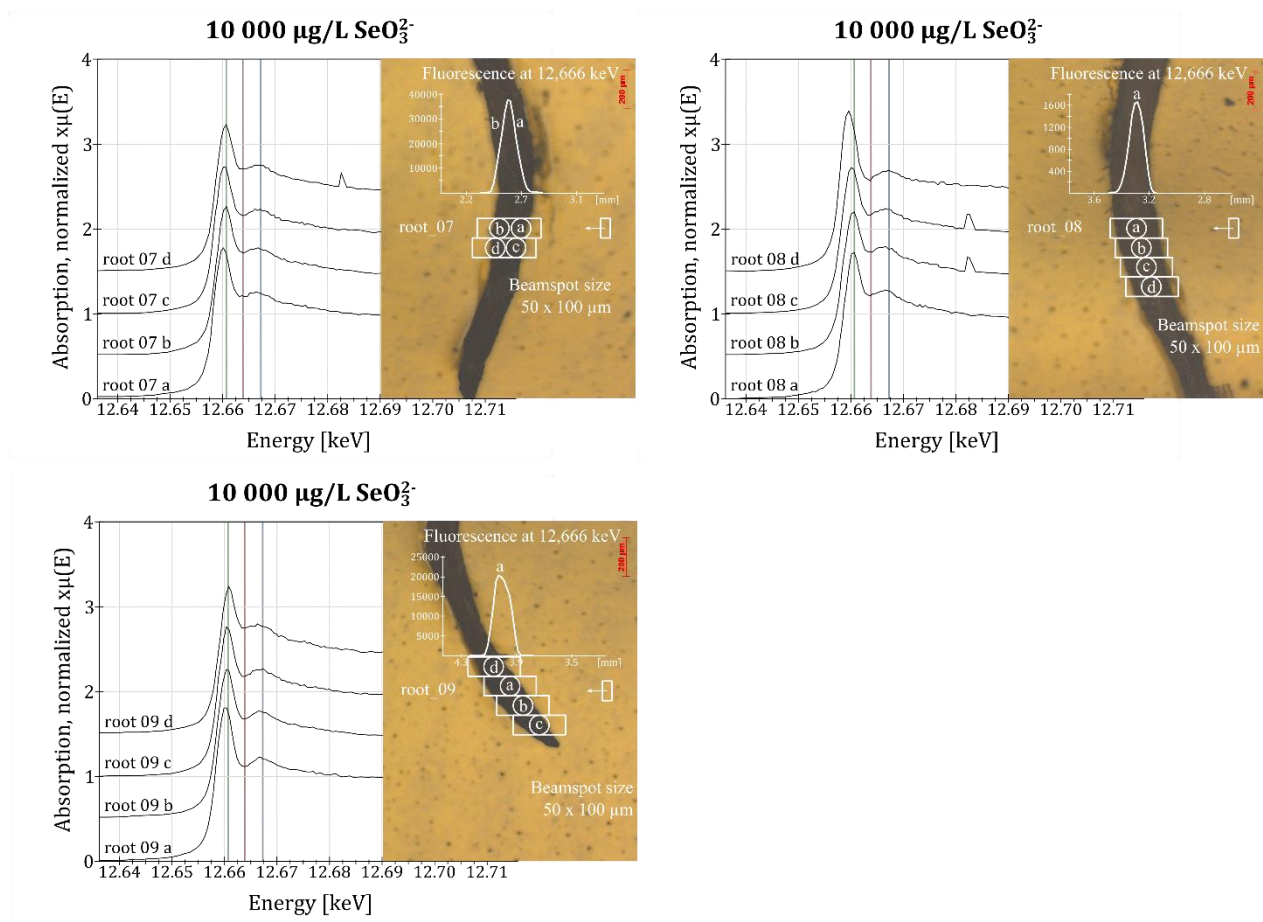
S23 Fig: all XANES spectra of each region of interest (ROI) on a rice plant treated with 10,000 \mu\text{g/L} Se as \text{Na}_2\text{SeO}_3 in nutrient solution
