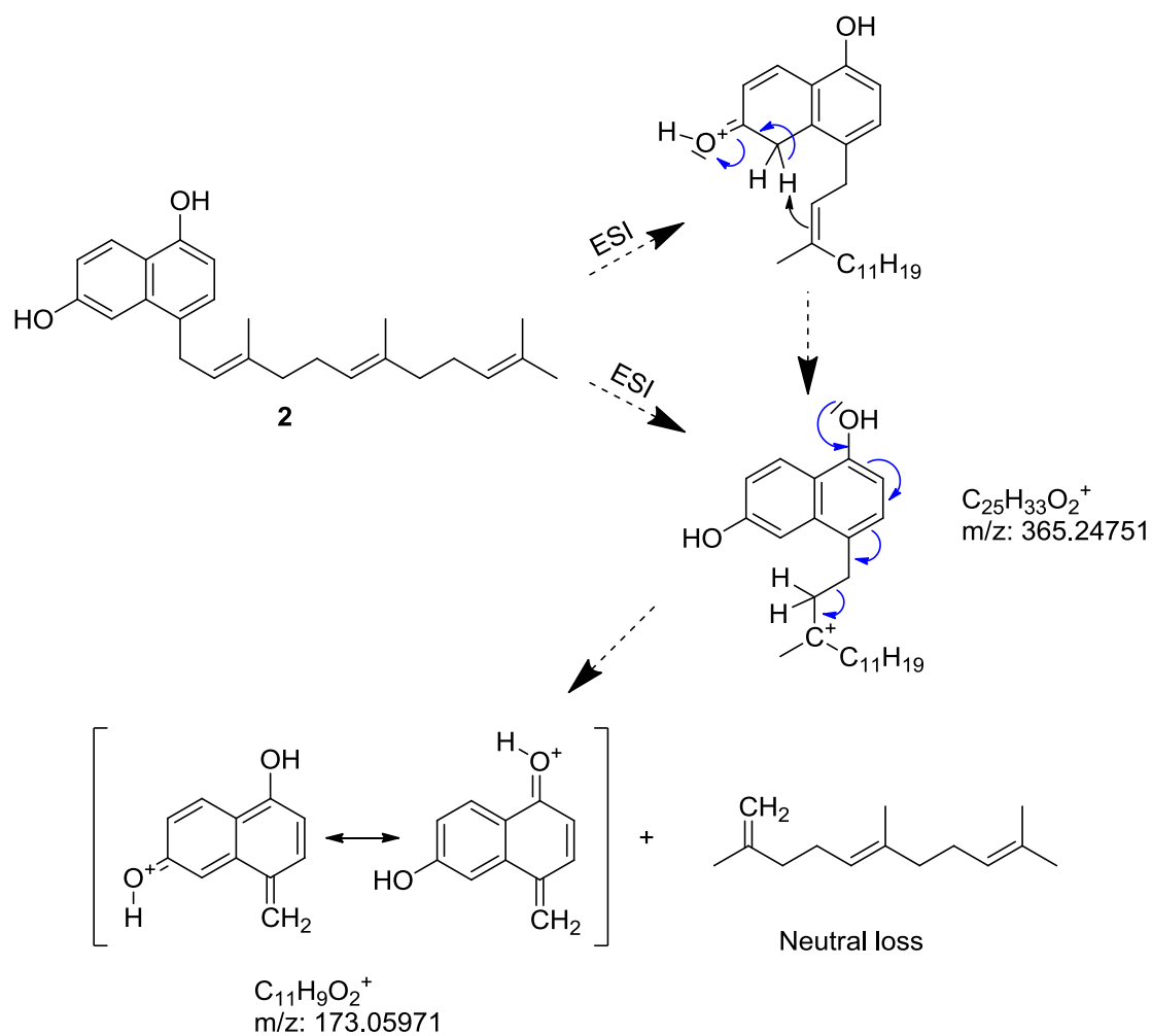
Figure S3. Potential protonation and proposed MS fragmentation mechanism of the product formed under catalysis of DzmP from 1,6-DHN and FPP, 4-[(2 E ,6 E )-3,7,11-trimethyl-2,6,10-dodecatrienyl]-naphthalene-1,6-diol ( 2 ).
