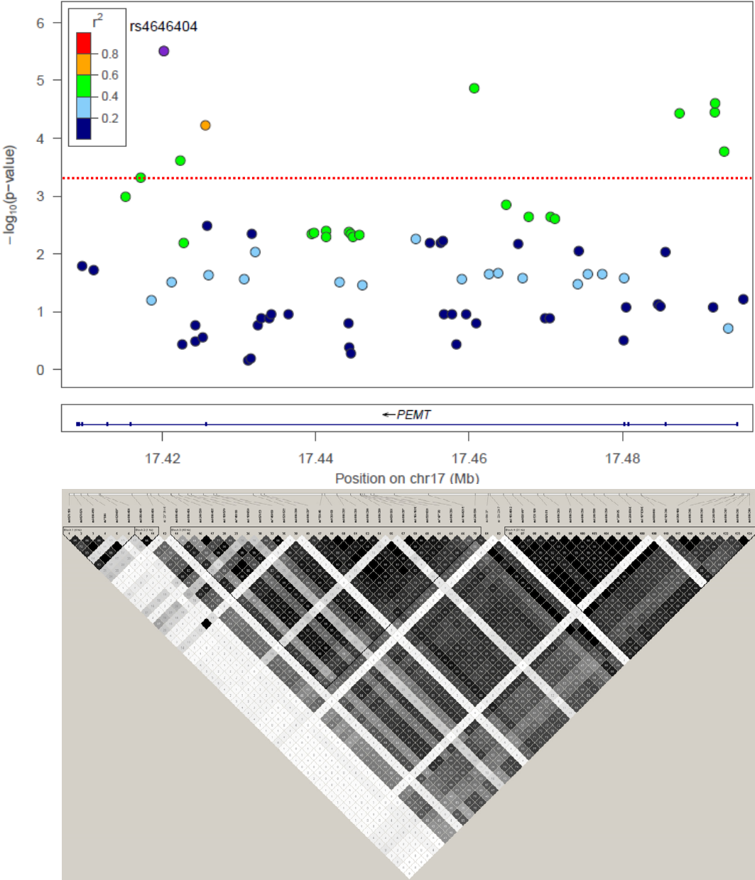
Figure S2: Linkage Disequilibrium among SNPs in PEMT gene. Top graph also indicates association of PEMT SNPs with WHR (adjusted for BMI) in Caucasian subjects from the GIANT consortium.
