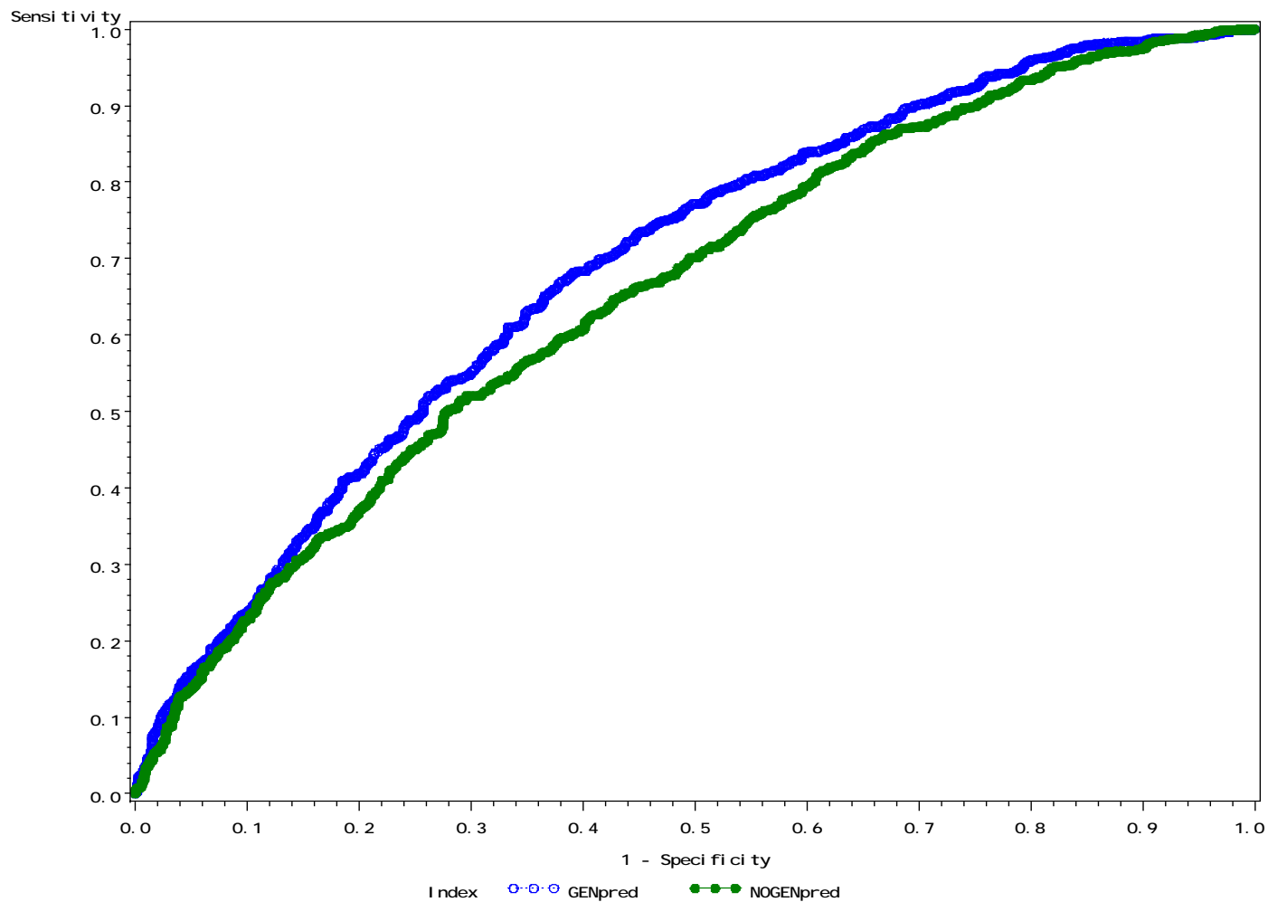
Figure S1. ROC curves for the prediction of prevalent hyperuricemia at baseline in SOS subjects with (blue line) and without (green line) the inclusion of SLC2A9 rs13113918 genotype in the model.
