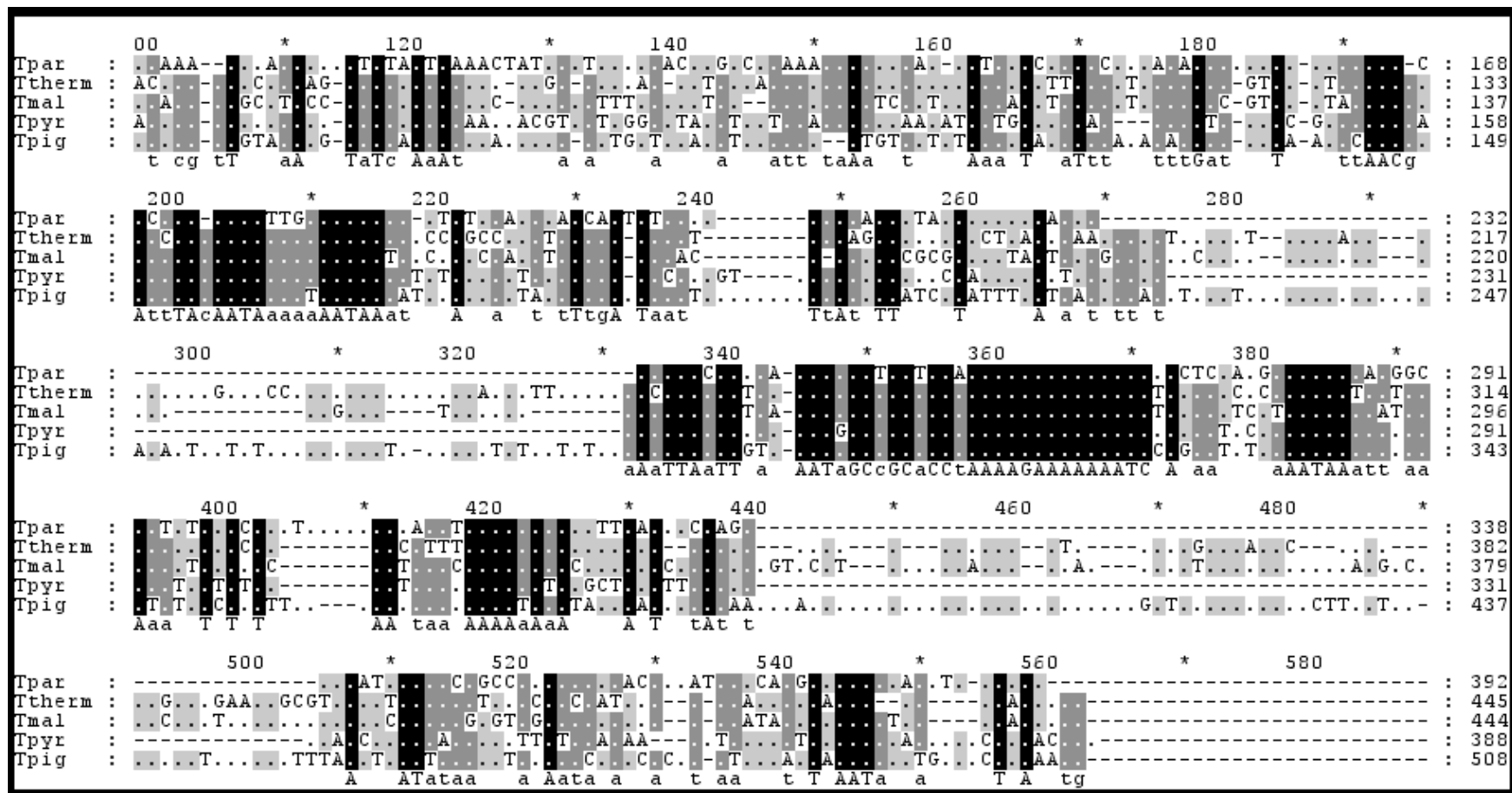
Figure S2- GeneDoc Nucleotide alignment of the cob and ymf77 intergenic region.
